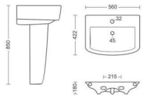
FULL PEDESTAL L422, W560, H850MM
