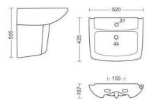
LOURET HALF PEDESTAL L425, W520, H505MM
