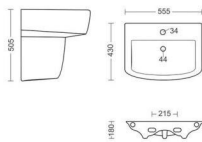
HALF PEDESTAL L430, W555, H505MM
