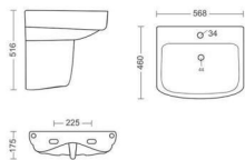
HALF PEDESTAL L460, W568, H516MM
